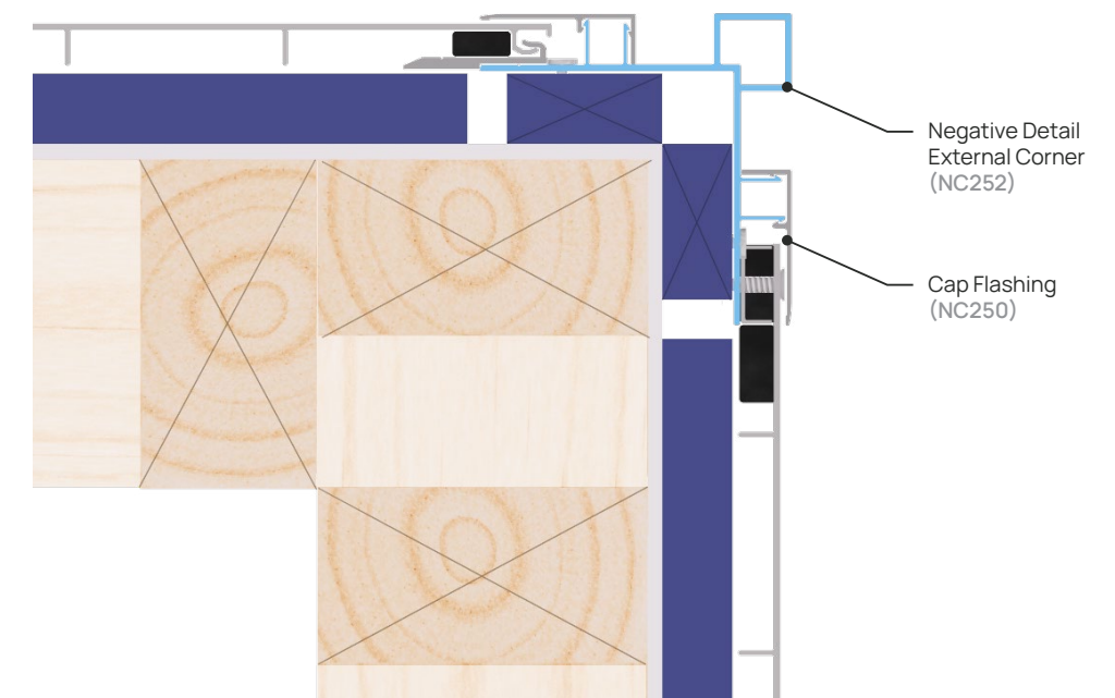
FIGURE 18: NEGATIVE DETAIL EXTERNAL CORNER FIXING
