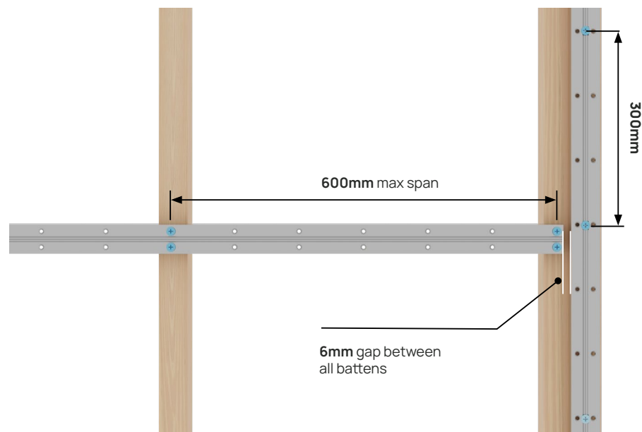
FIGURE 5: ALIBAT ON TIMBER FIXING
