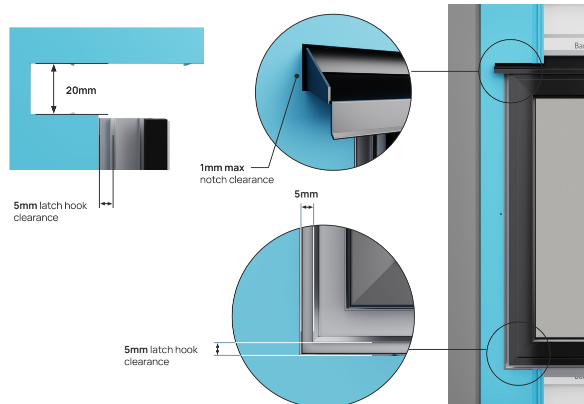
FIGURE 37. VERTICAL BOARD JOINERY NOTCH AND CLEARANCE REQUIREMENTS
