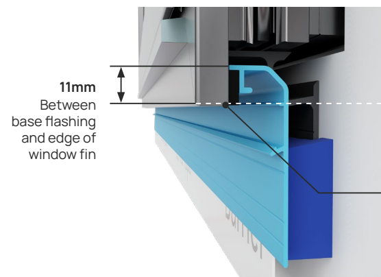
FIGURE 26. NC247 JOINERY BASE-FLASHING ALIGNMENT
