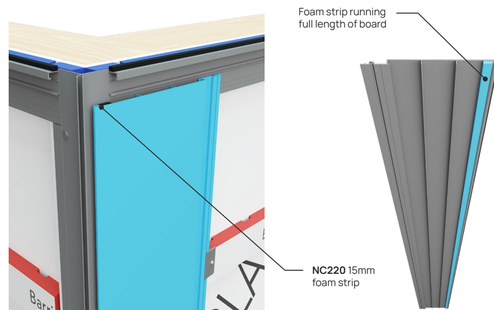
FIGURE 33. LOCATION OF 15MM FOAM STRIP
