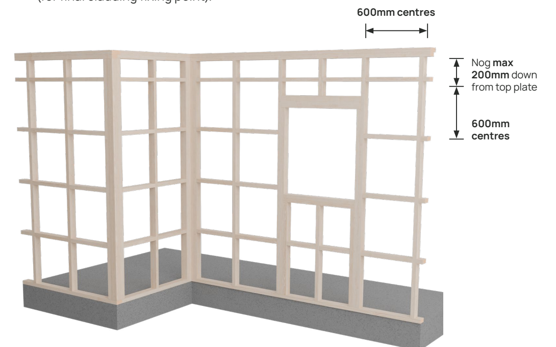
FIGURE 1. TYPICAL FRAMING CONFIGURATION FOR VERTICAL CLADDING
