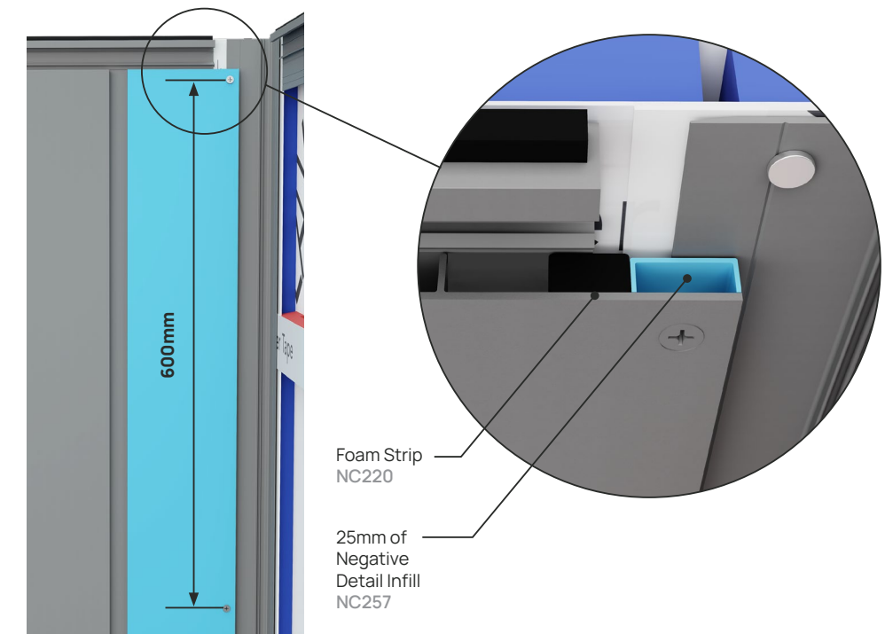
FIGURE 36. RIPPED BOARD FASTENING AND PACKER
