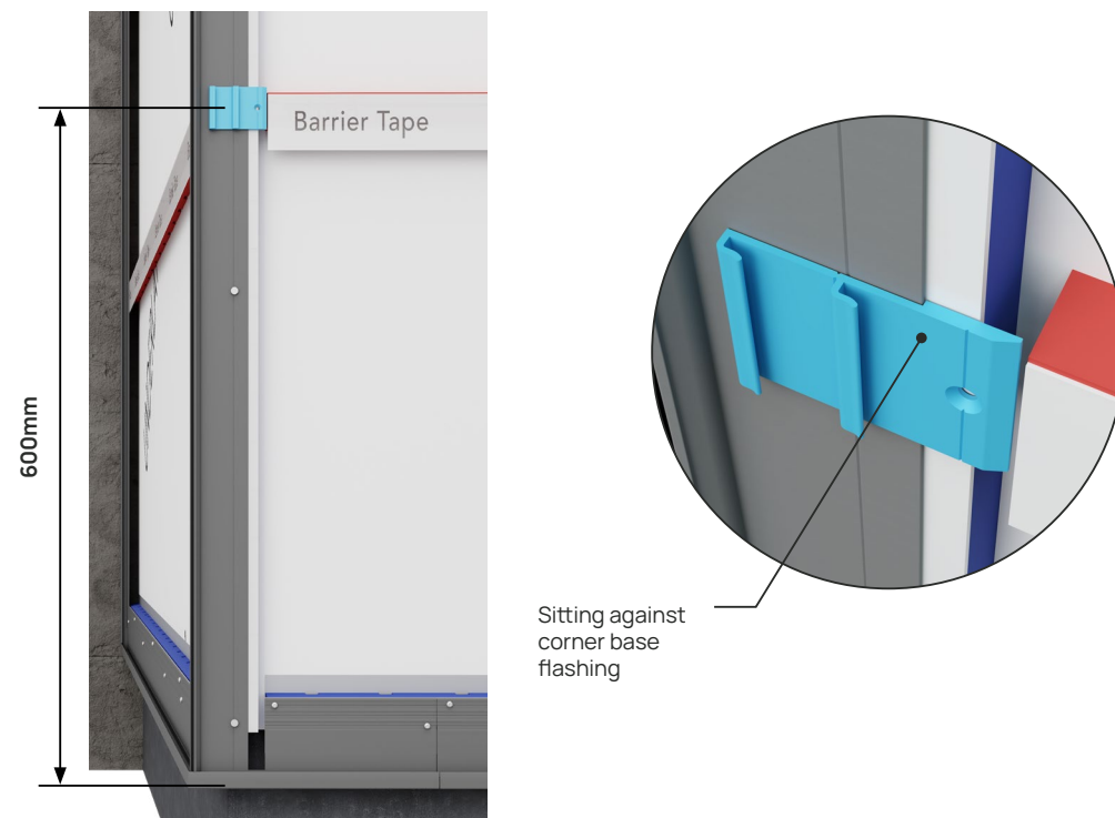
FIGURE 30. FIXING THE STARTER CLIP (NC232F)
