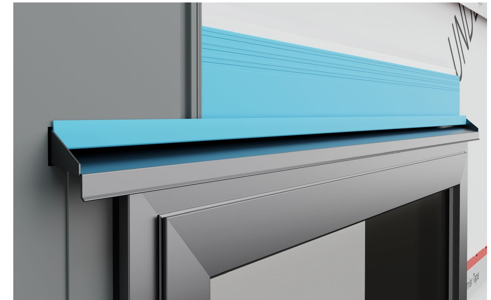
FIGURE 38. BASE CHANNEL FITTED ABOVE HEAD FLASHING - AFTER NOTCHED BOARD HAS BEEN INSTALLED
