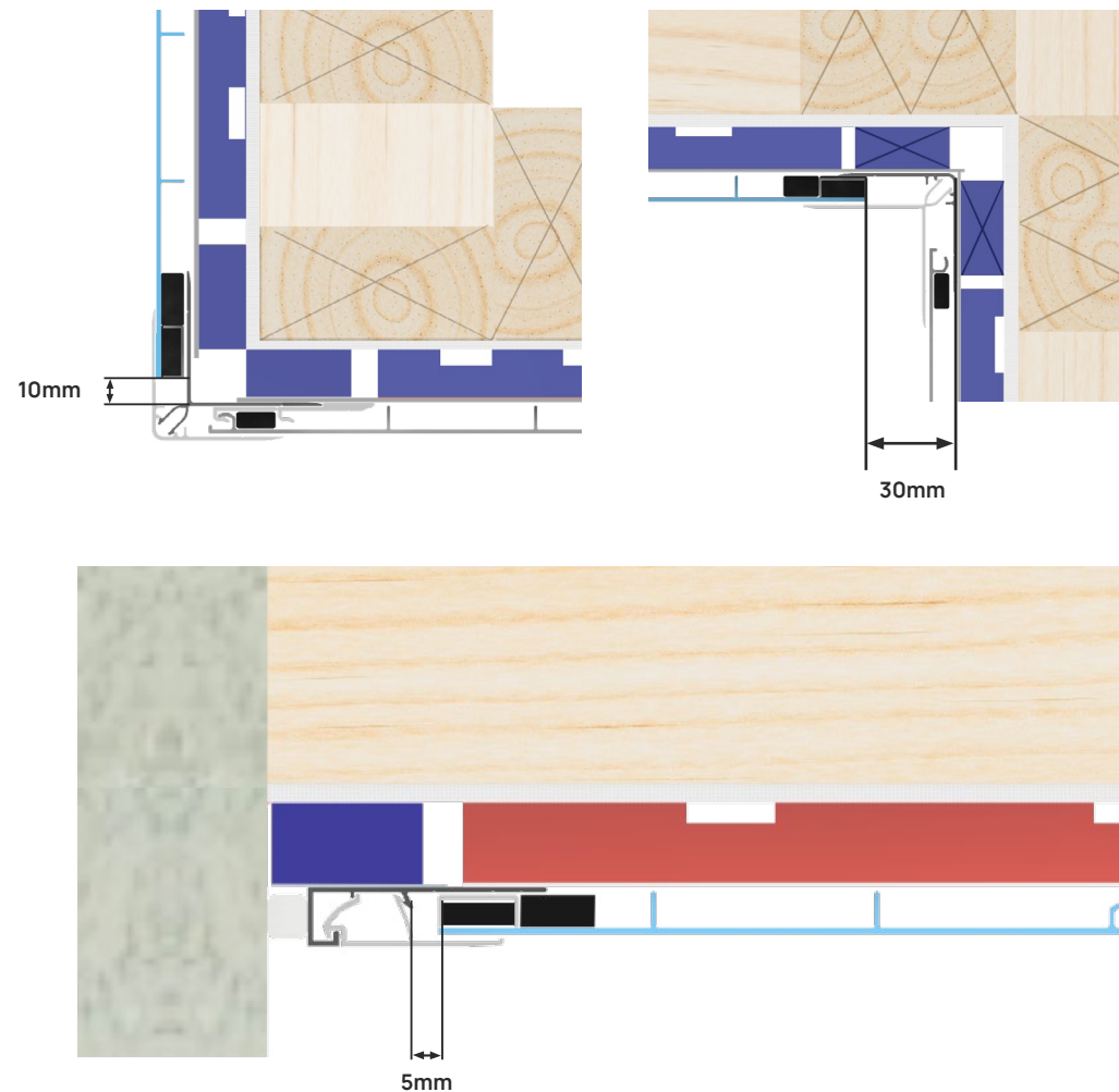
FIGURE 35. RIPPED BOARD CLEARANCES
