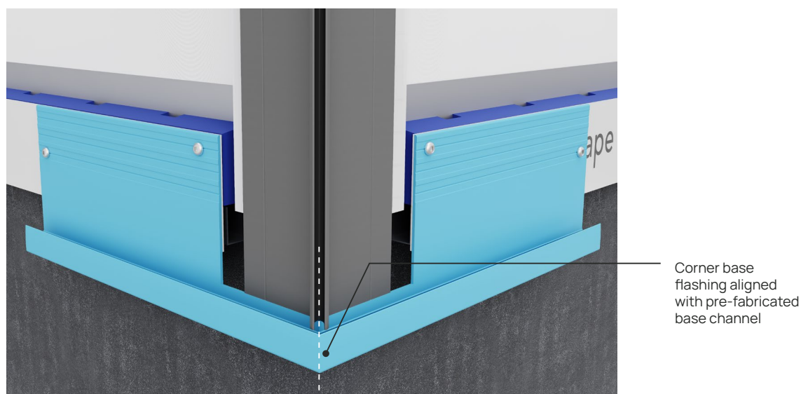
FIGURE 11: ALIGN THE CORNER FLASHING WITH THE BASE CHANNEL CORNER
