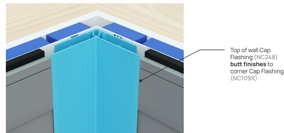
FIGURE 17: INTERNAL CORNER FIXING FIGURE (NC107X / NC109X)
