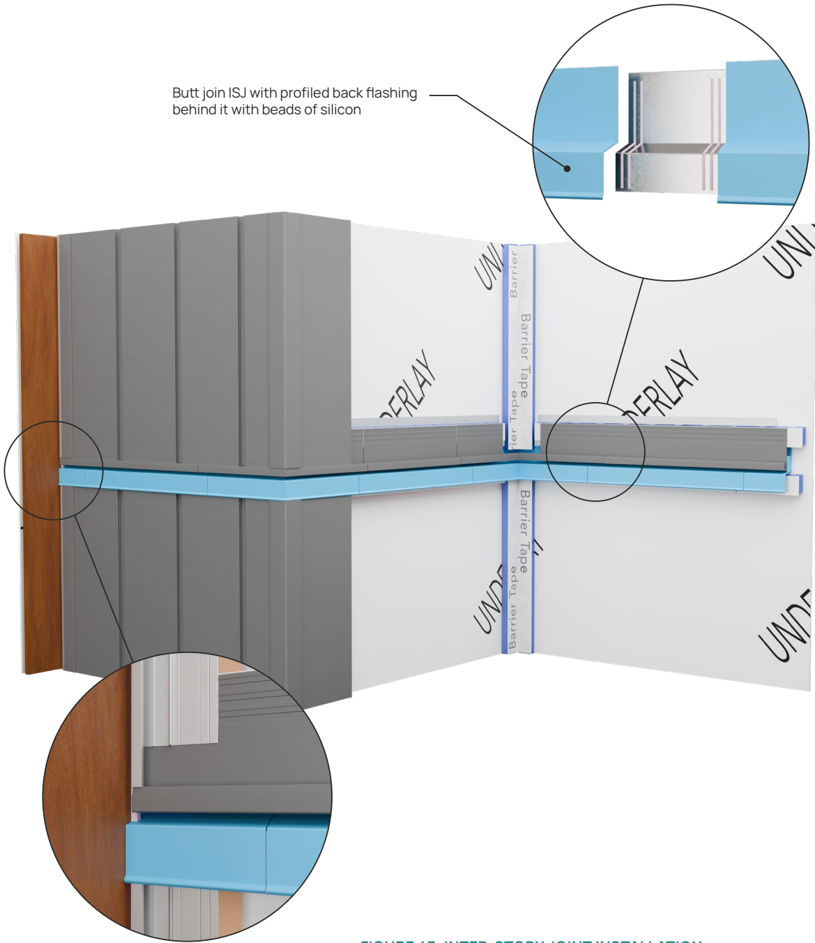
FIGURE 43. INTER-STORY JOINT INSTALLATION
