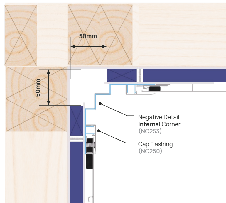
FIGURE 19. NEGATIVE DETAIL INTERNAL CORNER FIXING
