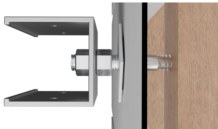
FIGURE 42. LAG BOLT PENETRATION
