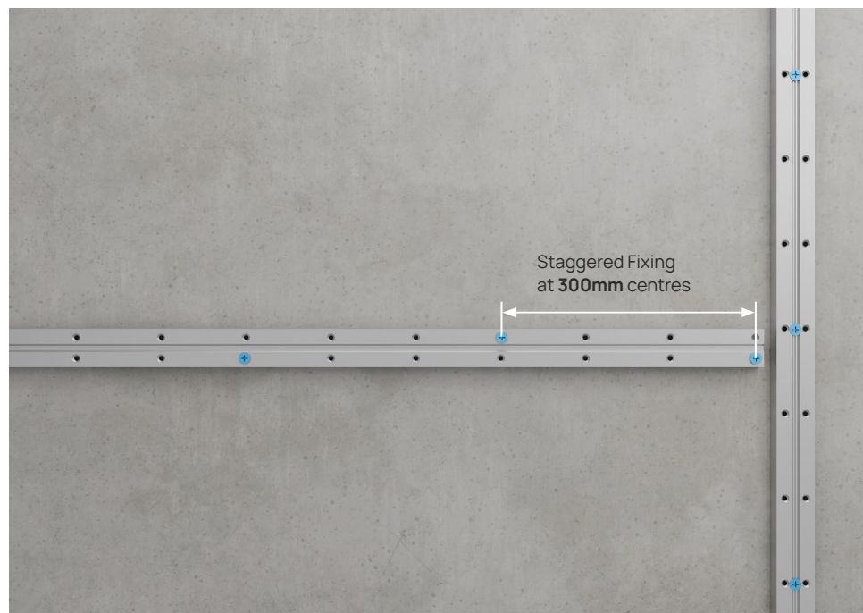
FIGURE 6: ALIBAT ON CONCRETE FIXING
