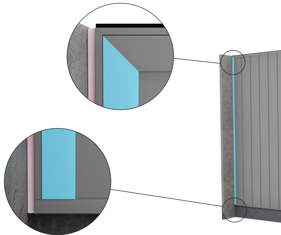
FIGURE 23. VERTICAL CLADDING TERMINATION CAP FLASHING INSTALLATION
