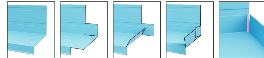
FIGURE 9: JOINERY HEAD FLASHING PREPARATION
