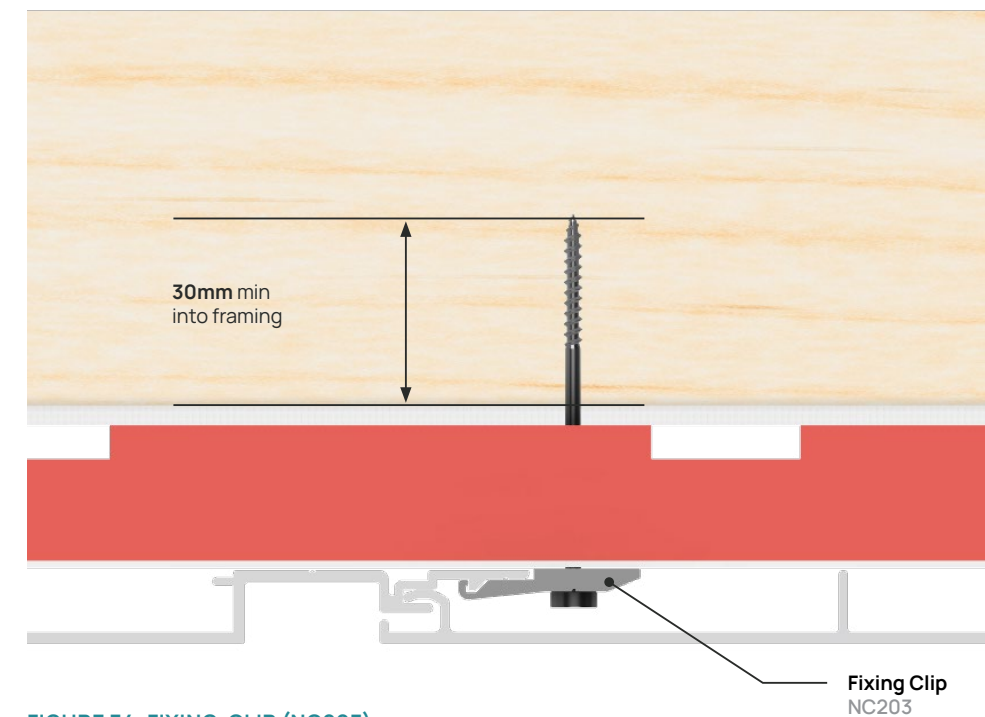
FIGURE 34. FIXING-CLIP (NC203)
