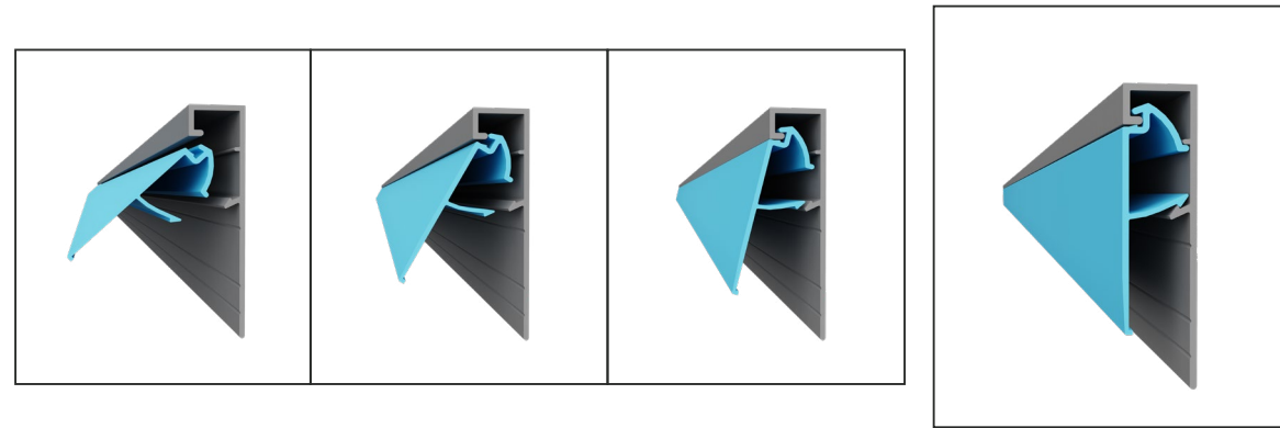
FIGURE 20. "ROTATE-IN" NC247T TERMINATION FLASHING ASSEMBLY
