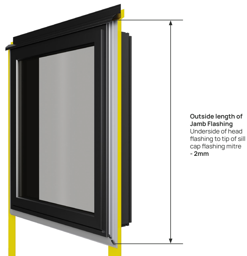
FIGURE 29. JAMB CAP FLASHING LENGTH
