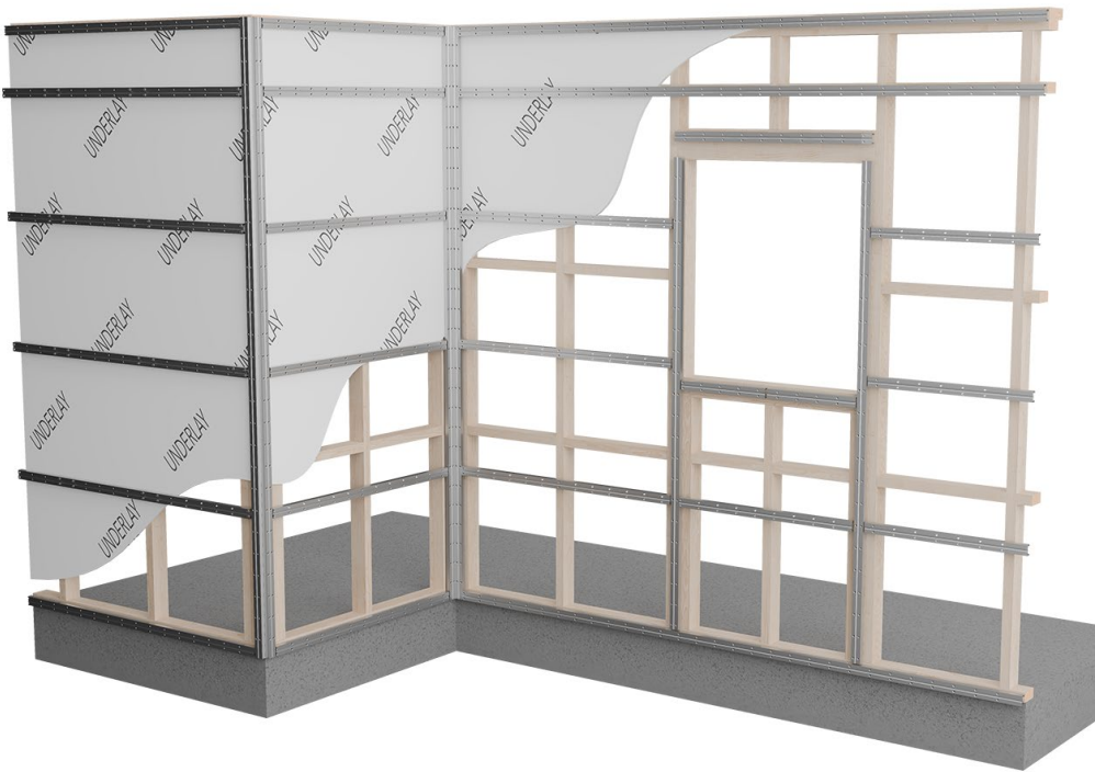
FIGURE 4. TYPICAL ALIBAT CONFIGURATION
