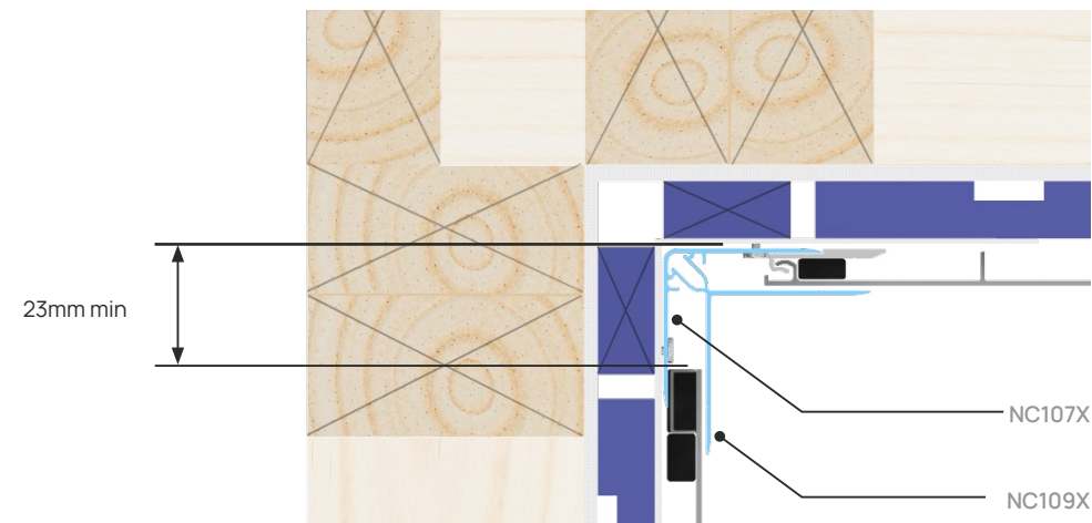
FIGURE 16: INTERNAL CORNER FIXING FIGURE (NC107X / NC109X)
