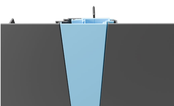
FIGURE 40. MONO50 MAINTENANCE JOINT
