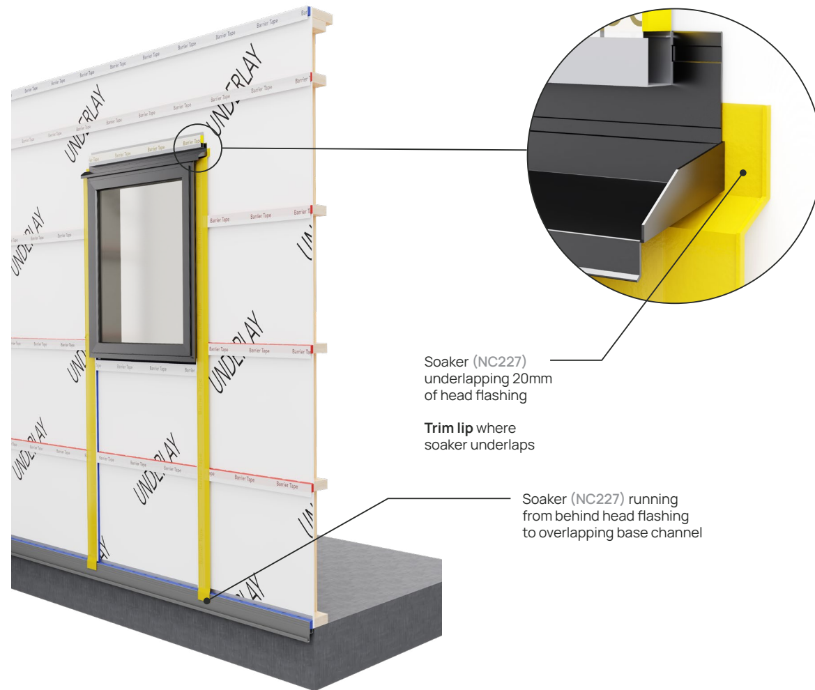
FIGURE 8: SOAKER INSTALLATION
